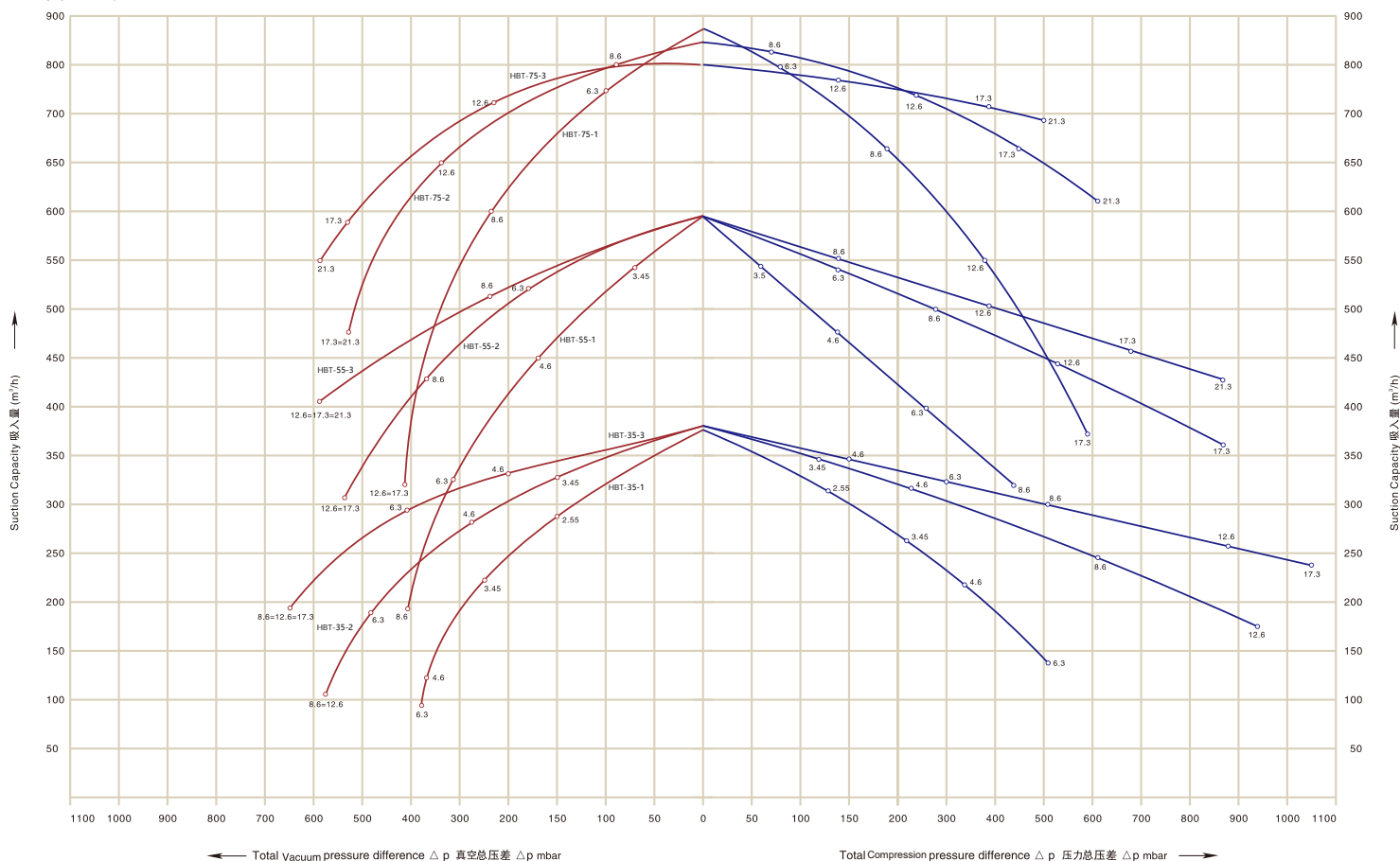
Vacuum Compression Selection Diagram 真空压缩图表 60Hz
